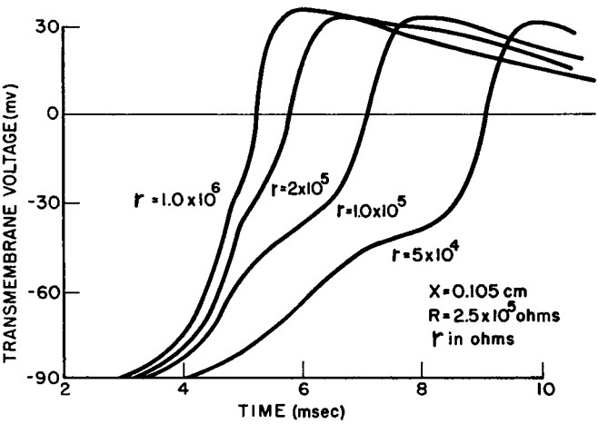
FIGURE 8 B Transmembrane voltage vs. time. x = 0.105 cm. R = 2.5 \times 10^5 \Omega . r in \Omega .
