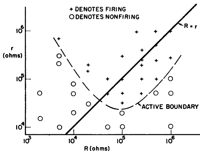
FIGURE 9 Summary of firing results. + denotes firing. O denotes nonfiring.
